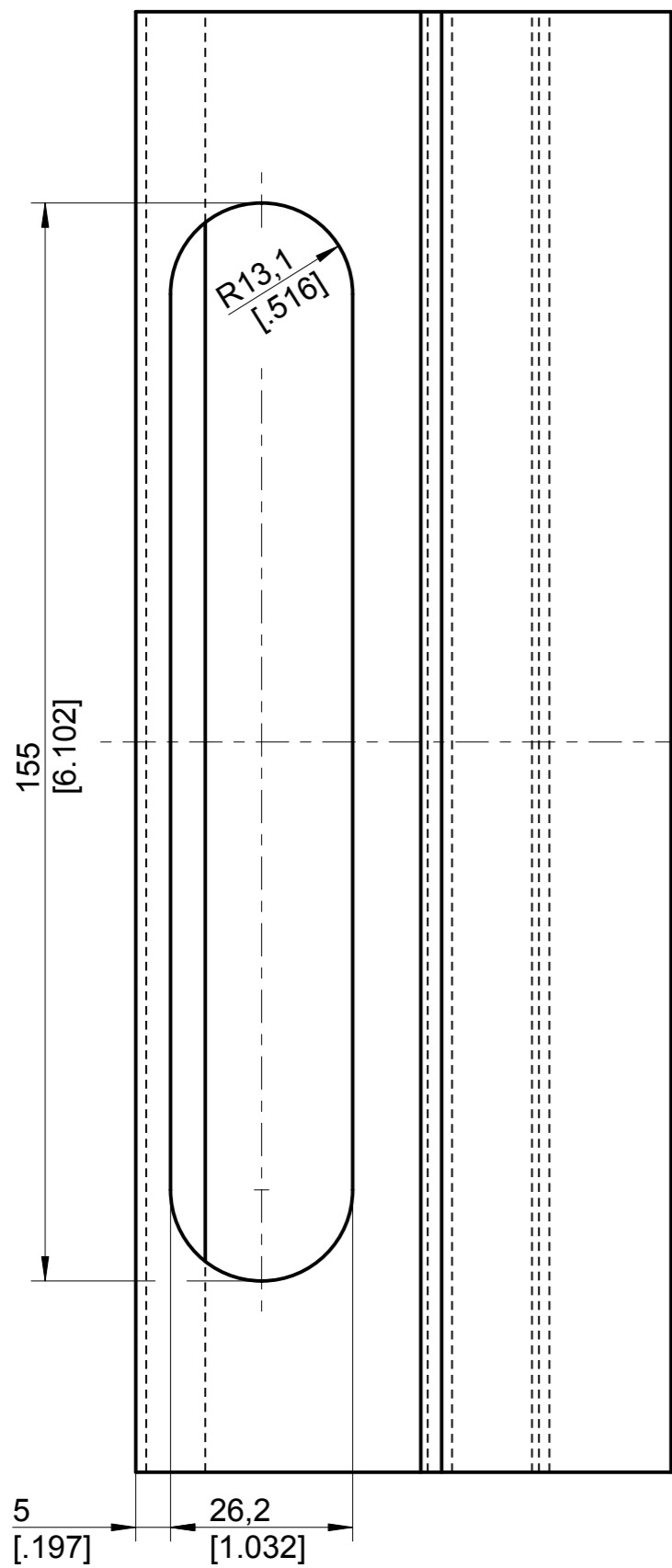
template steel frame
